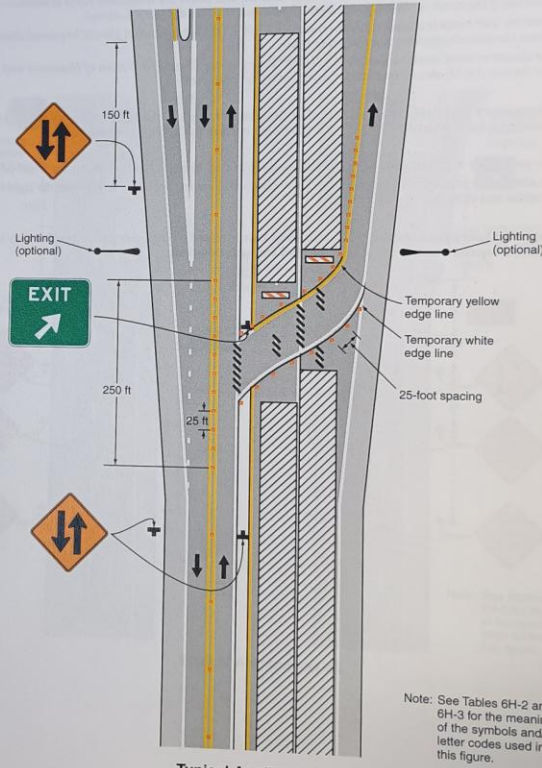
Typical Application 41
