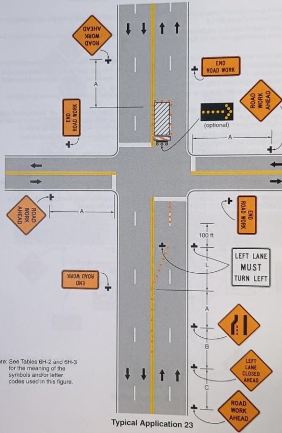
Figure 6H-23. Left-Hand Lane Closure on the Far Side of an Intersection (TA-23)
