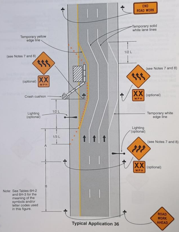
Figure 6H-36. Lane Shift on a Freeway (TA-36)
