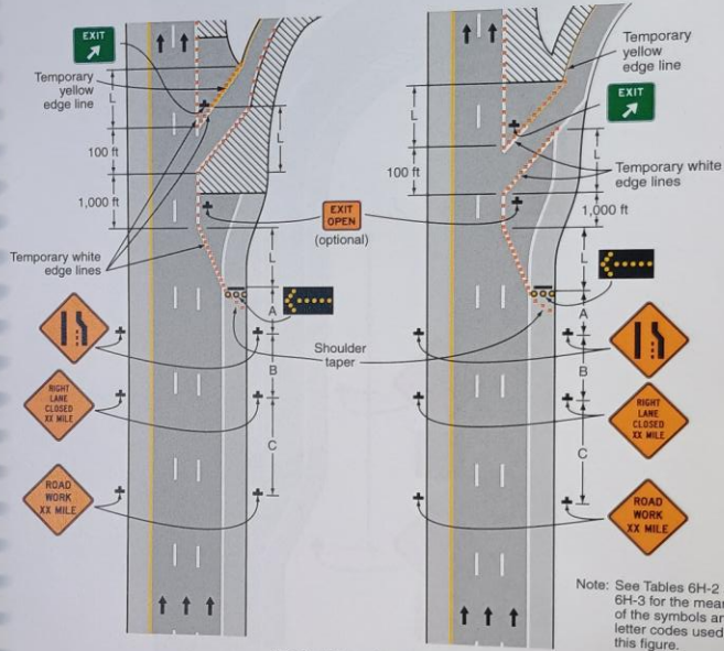
Typical Application 42
