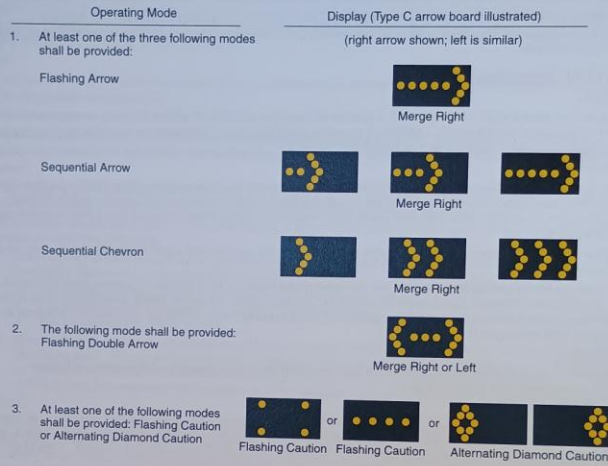
Figure 6F-6. Advance Warning Arrow Board Display Specifications
