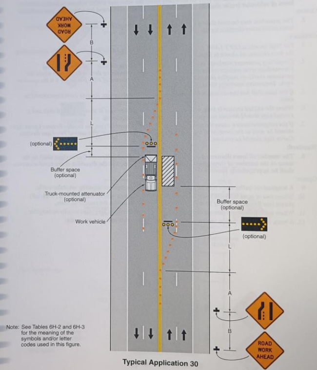
Figure 6H-30. Interior Lane Closure on a Multi-Lane Street (TA-30)
