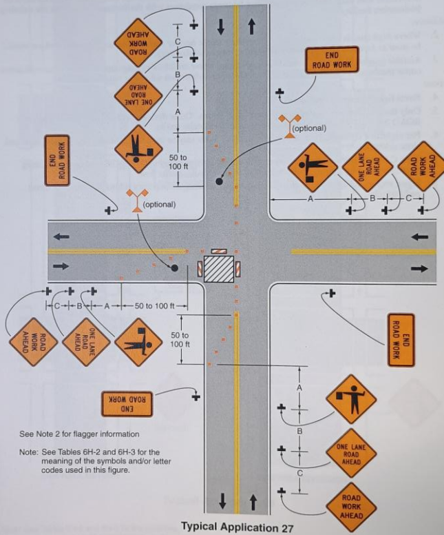
Typical Application 27
