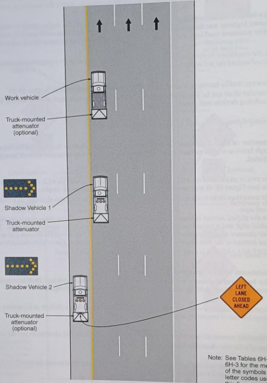
Typical Application 35
