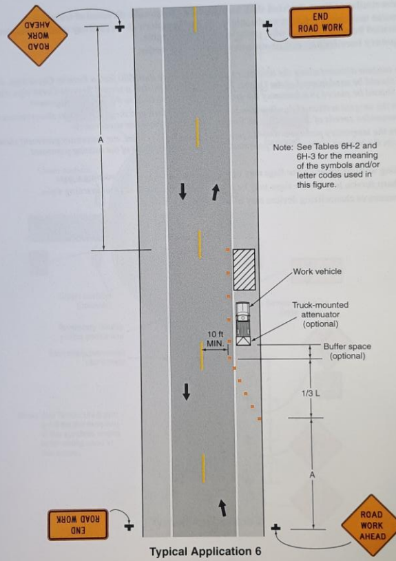
Typical Application 6
