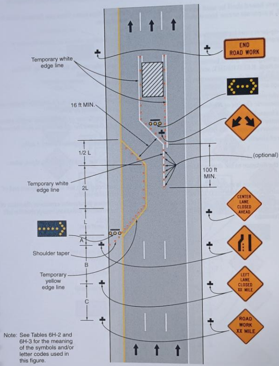
Typical Application 38
