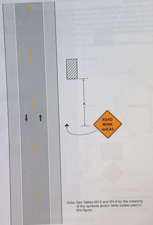
Typical Application 1
