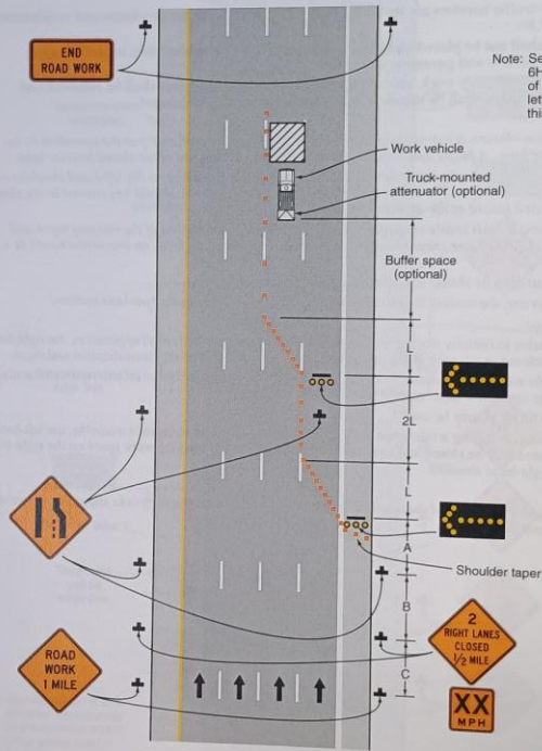
Typical Application 37
