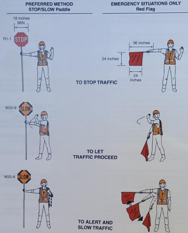
Figure 6E-3. Use of Hand-Signaling Devices by Flaggers
