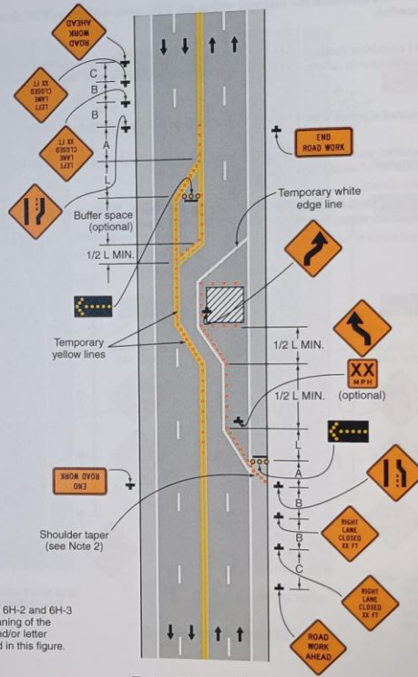
Typical Application 32
