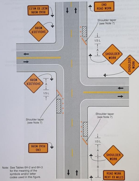
Typical Application 3
