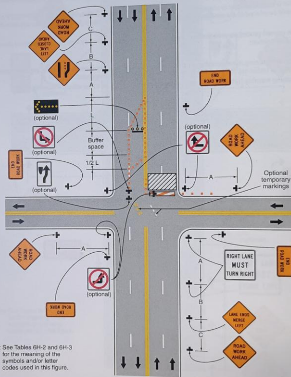
Typical Application 24
