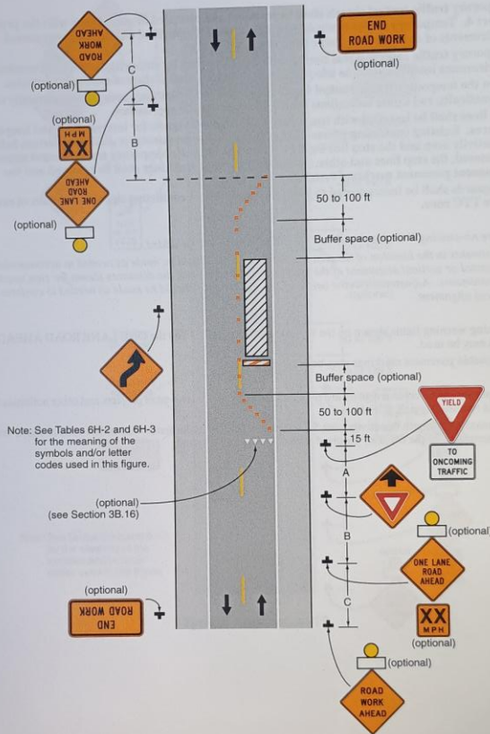
Typical Application 11
