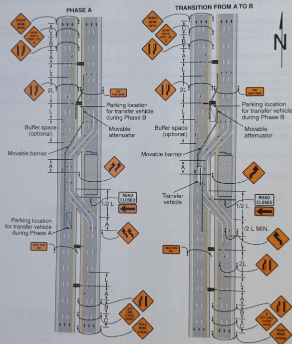
Typical Application 45
