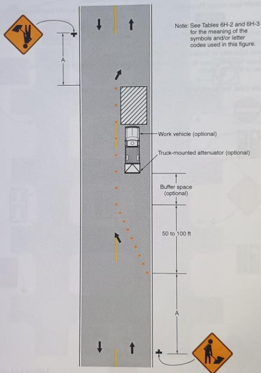
Typical Application 18
