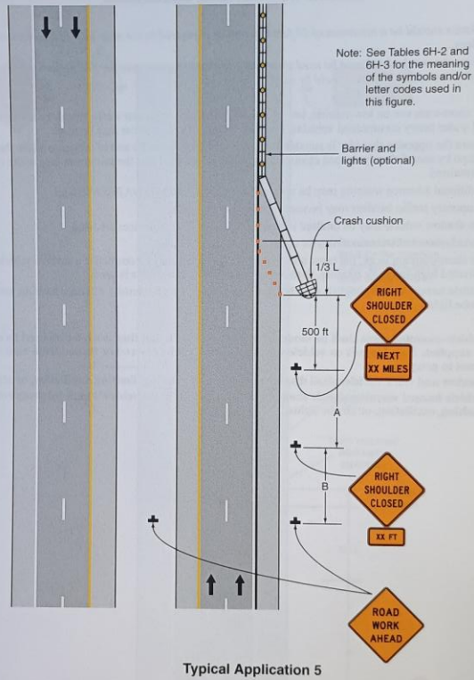
Figure 6H-5. Shoulder Closure on a Freeway (TA-5)
