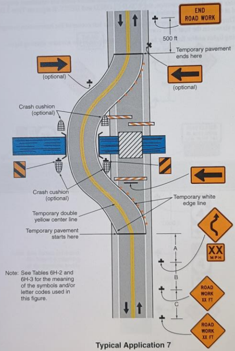
Typical Application 7
