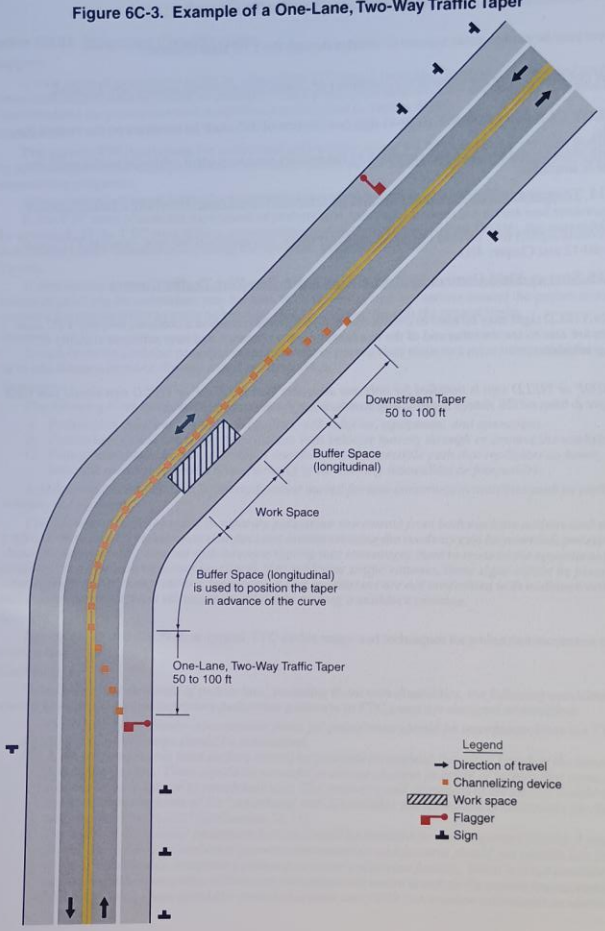
Figure 6C-3. Example of a One-Lane, Two-Way Traffic Taper
