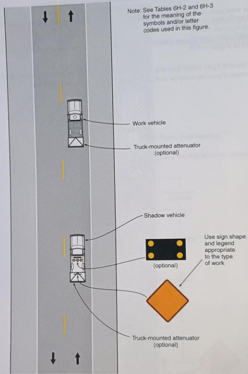
Typical Application 17
