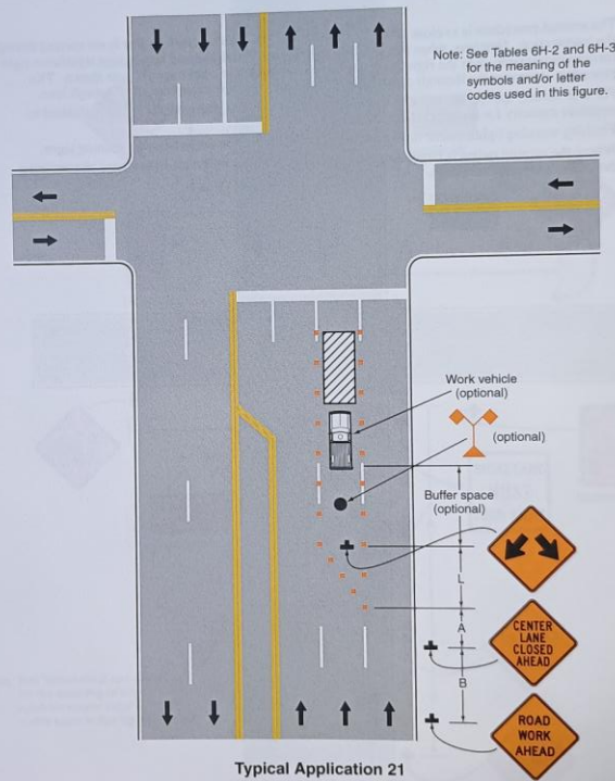
Typical Application 21
