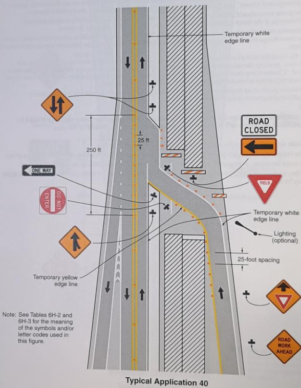
Figure 6H-40. Median Crossover for an Entrance Ramp (TA-40)
