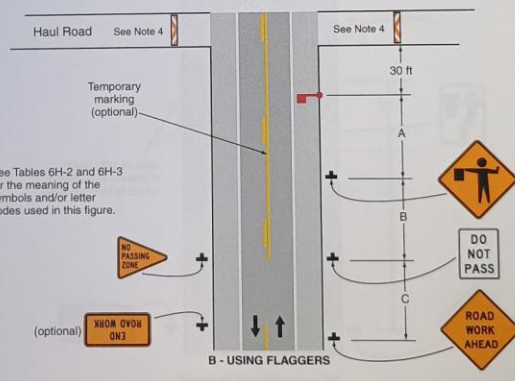
Typical Application 14
