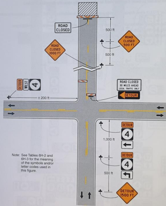
Typical Application 8
