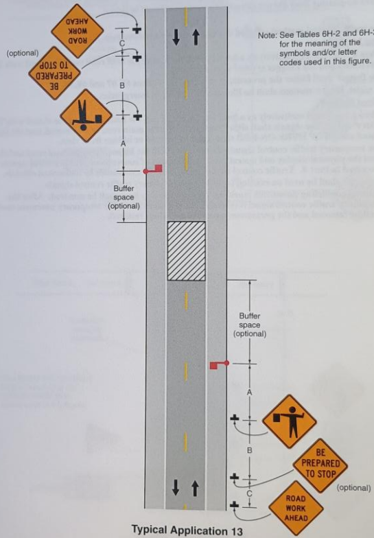
Typical Application 13
