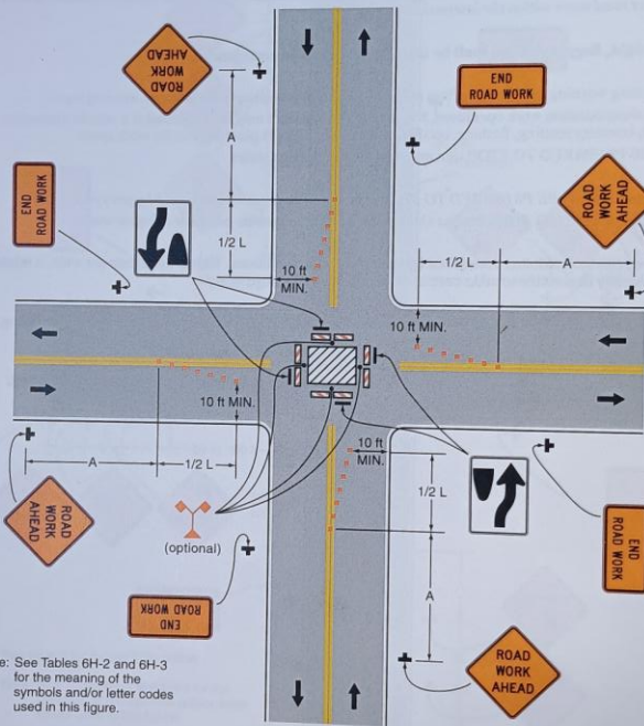
Typical Application 26
