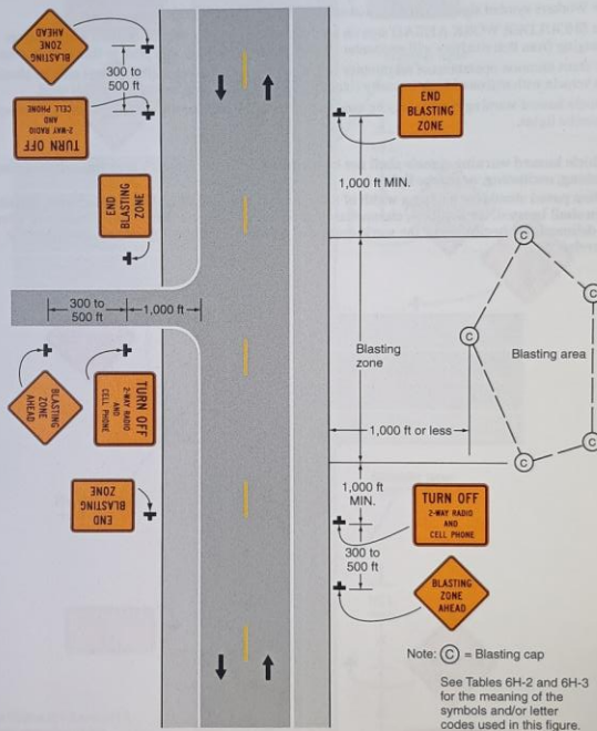
Typical Application 2
