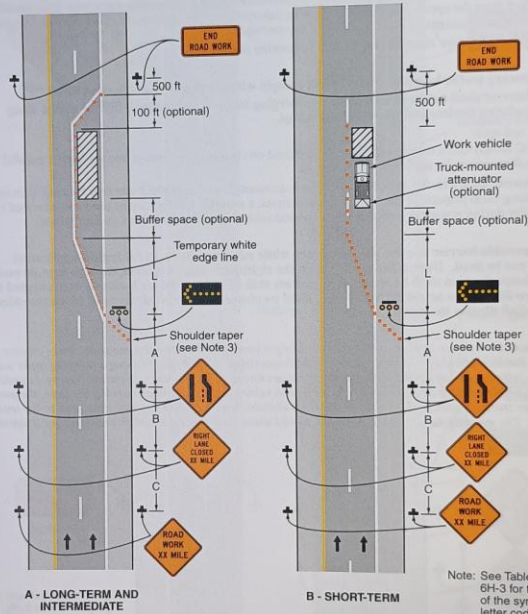
Typical Application 33
