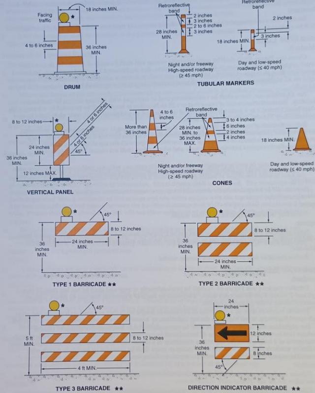
Figure 6F-7. Channelizing Devices
